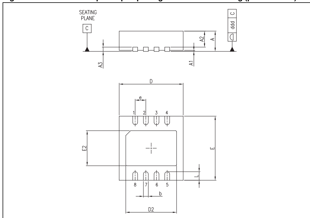
Figure 18. DFN8 3 x 3 exposed pad package mechanical drawing (pitch 0.5 mm)
