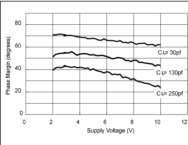
Figure 11. Phase margin vs. V_{CC} C_L = 30, 130 and 250 pF
